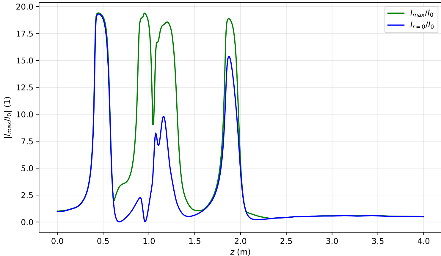
I_{max}(x = 0, y = 0, z)/I_0 , P_{in}=5.7P_{cr} , noisy input, artificial time
